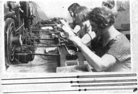
Eisler electric butt welders for lead-in wires were in 1921 the first such machines used by the independent lamp-makers.
